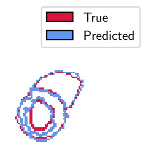
segmentations
